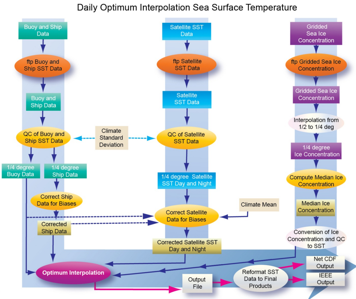
Figure 1: OISST Routine Processing flow. Not all ancillary data are shown
